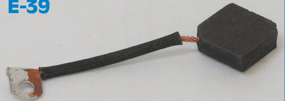
Dimensions: 6.5mm T X 19.5mm W X 22mm L x 51mm LL
